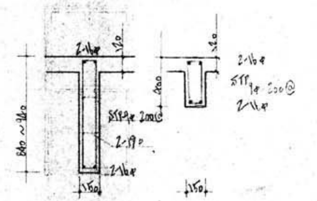
(R階梁伏図) RB
